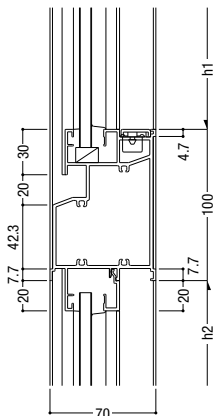
130 FIX / FIX
