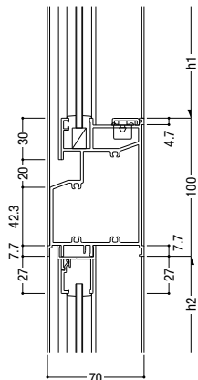
129 FIX / FIX
