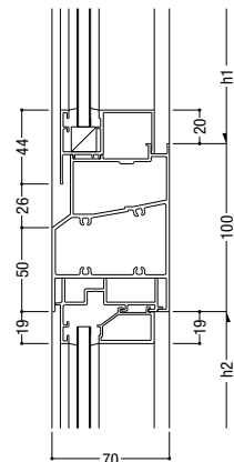
132 FIX / FIX
