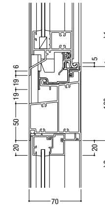
124 FIX / FIX
